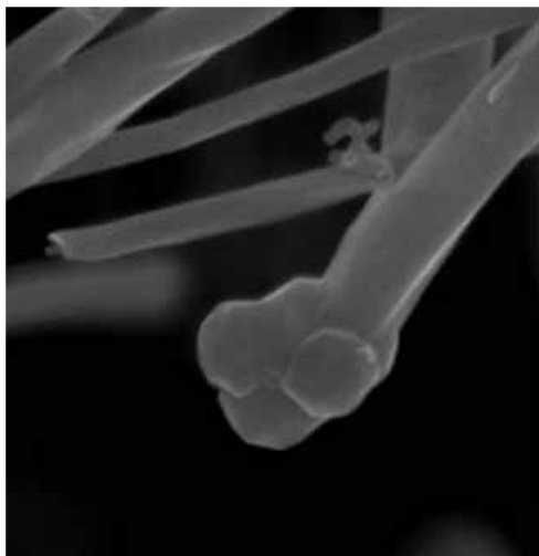
High-Resolution Scanning Electron Micrograph of Single Walled Carbon Nanotubes, taken by Rory Brimecombe as part of his PhD studies.
